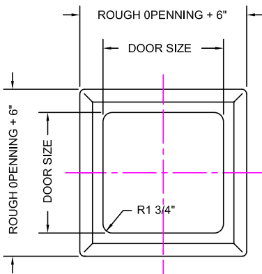
Drop-in Access Panel -Type Panel Elevations
