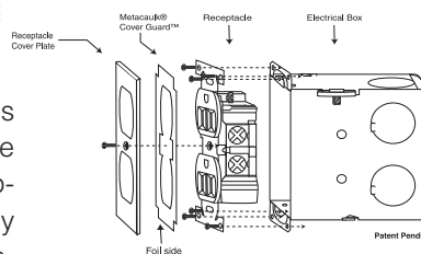
Installation of Single Receptacle
