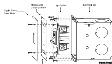
Installation of Single Electrical Switch
