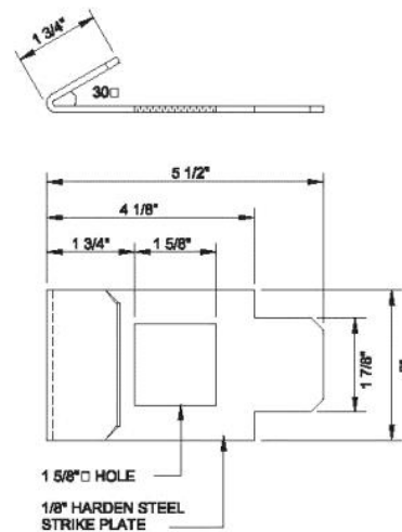
STRIKE PLATE 3" = 1'-0"
