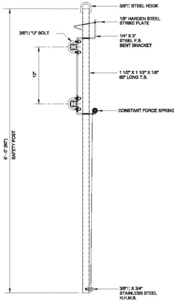
SAFETY POST 1" = 1'-0"
