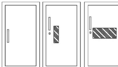
S21 - Solid with pull L22 - Solid with pull and Saf-T-Lok L24 - Solid with cylinder key lock/no pull (L22,24 not shown) B10 - Vertical acrylic view window. 5" x 5" with pull, and Saf-T-Lok A - Horizontal duo panel with pull and Saf-T-Lok
