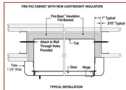
TYPICAL INSTALLATION
