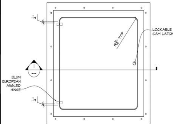
REFLECTED PLAN Scale: NTS
