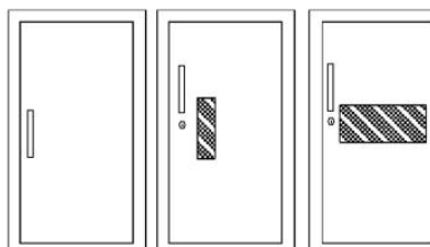
S21 - Solid with pull L22 - Solid with pull and Saf-T-Lok L24 - Solid with cylinder key lock/no pull (L22,24 not shown) B10 - Vertical acrylic view window 5" x 5" with pull, and Saf-T-Lok A - Horizontal duo panel with pull and Saf-T-Lok
