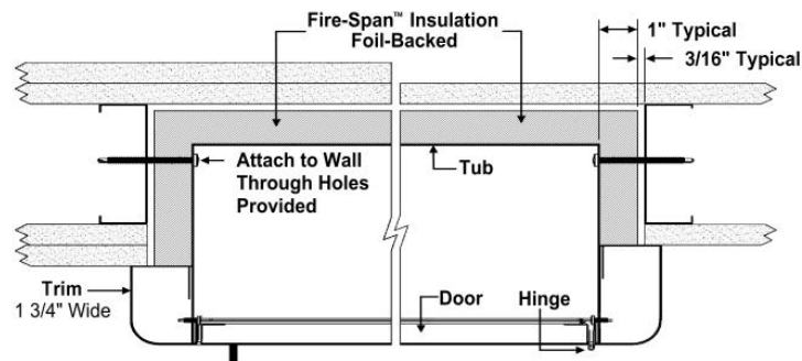
TYPICAL INSTALLATION
