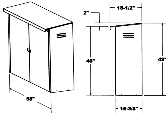
HECIG OR HECIR CABINET WITH OPTIONAL LOCKING CHROME HANDLE
